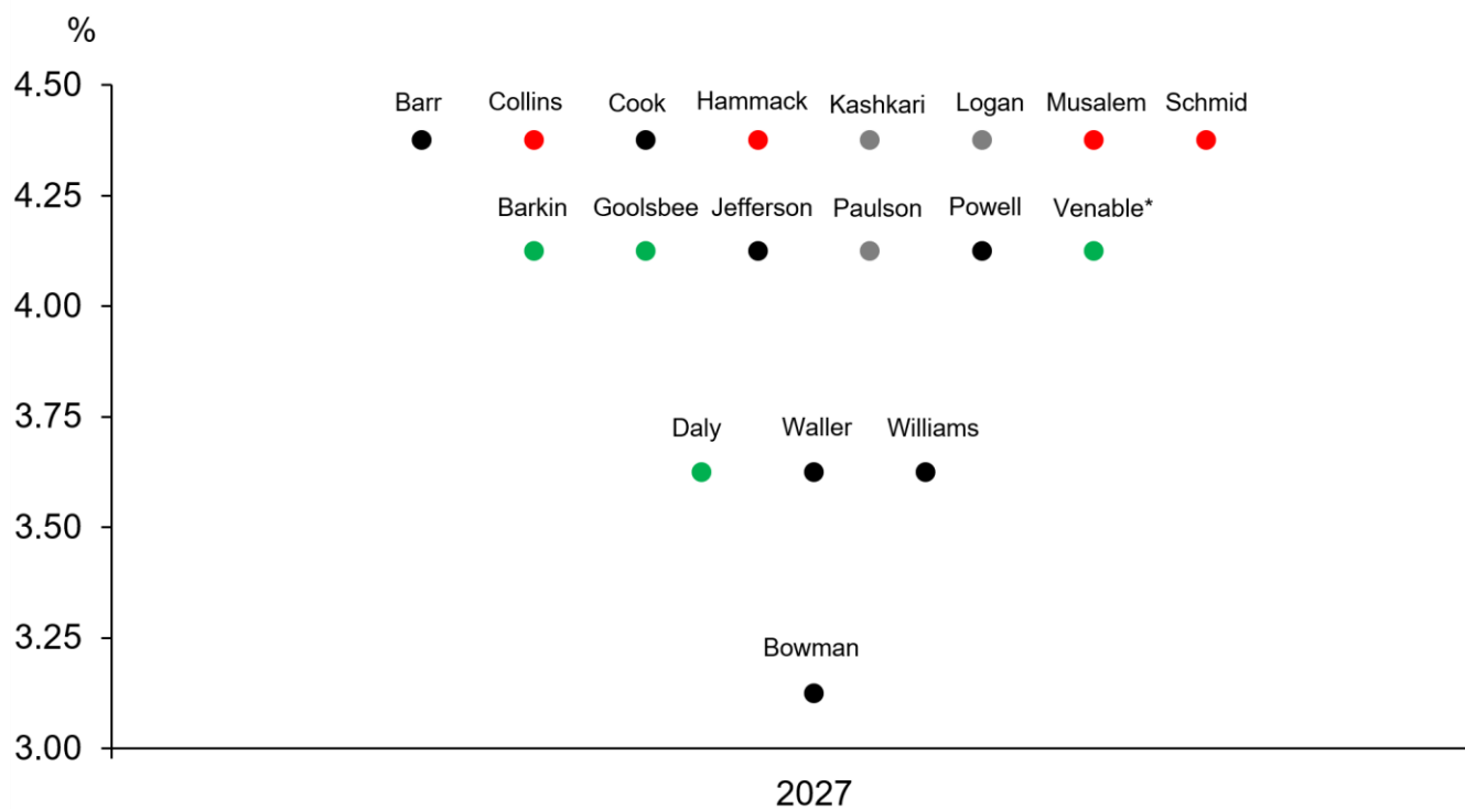
Figure 2: DB ID of the 2027 dots in September SEP
