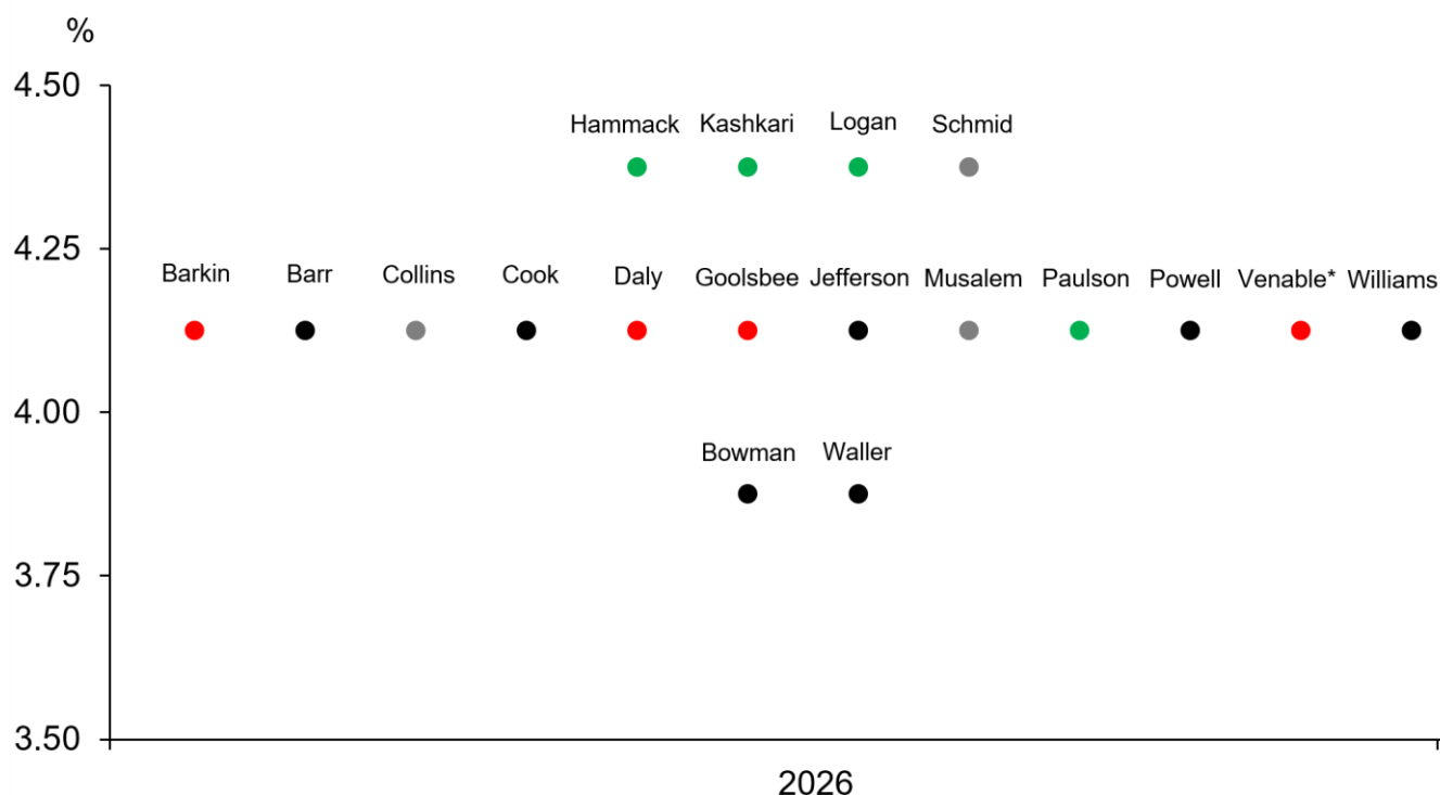
Figure 1: DB ID of the 2026 dots in September SEP
